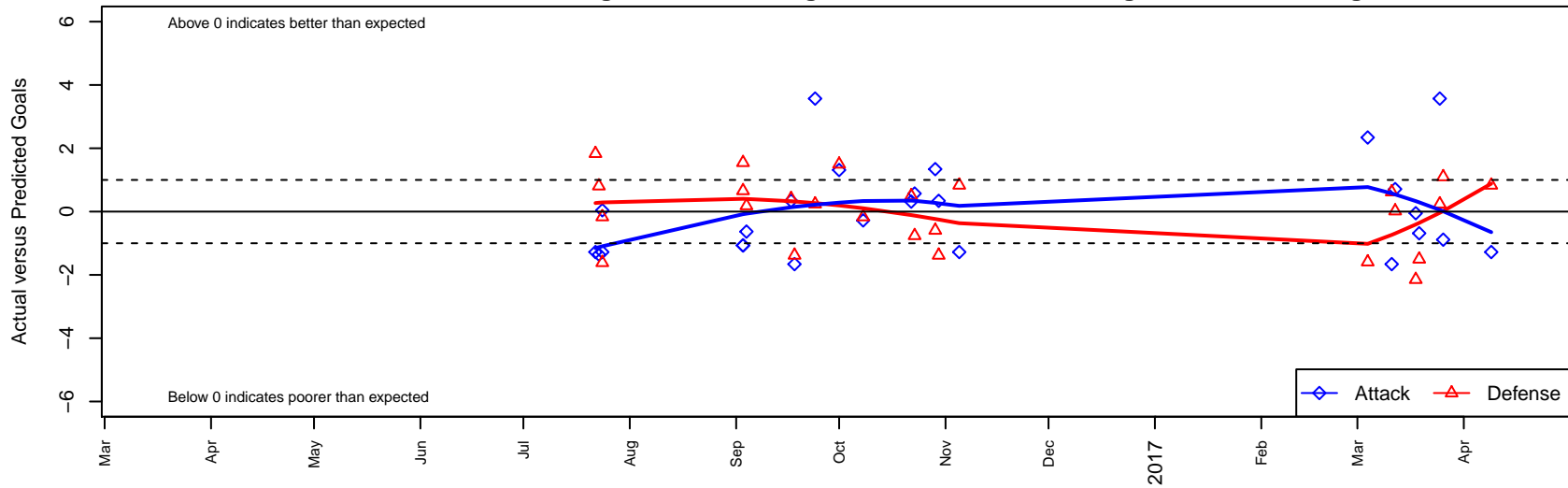
ASE Emerald G03 Dots are actual minus expected GF (blue circles) and GA (red triangles). Blue line is smoothed change in attack strength. Red is smoothed change in defense strength.
